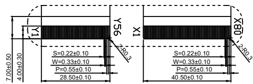
DETAIL B
