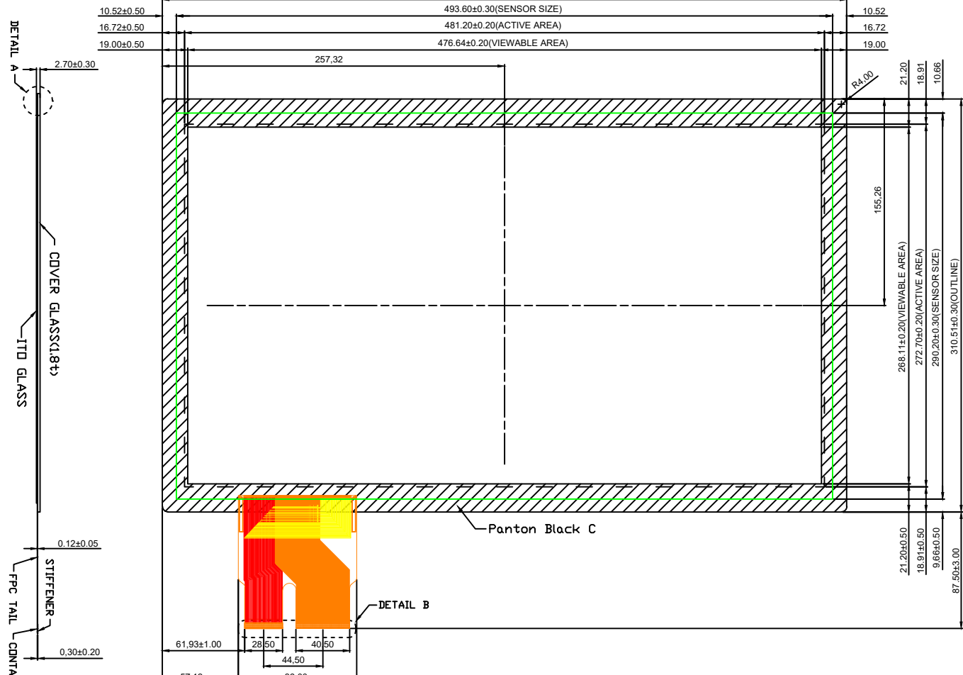
DETAIL B
