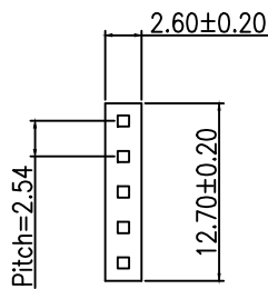
HOUSING (LOCKING)
